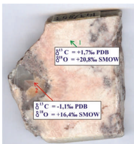
Figure 5: Isotopic composition of primary dolomite (green 1) and relatively late magnesite (red 2) in the apatite-bearing Precambrian carbonate ores of the Seligdar deposit, Yakutia.
