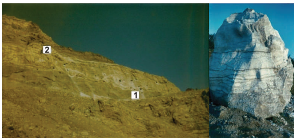
Figure 2: Liadzhvardara lazurite deposit, the Pamir Mountains. Separate layer (left) of dolomite marble (between point 1 and 2) with lazurite undergrounds (black points within marble layer), inner structure of salt-bearing dolomite marble (right).
