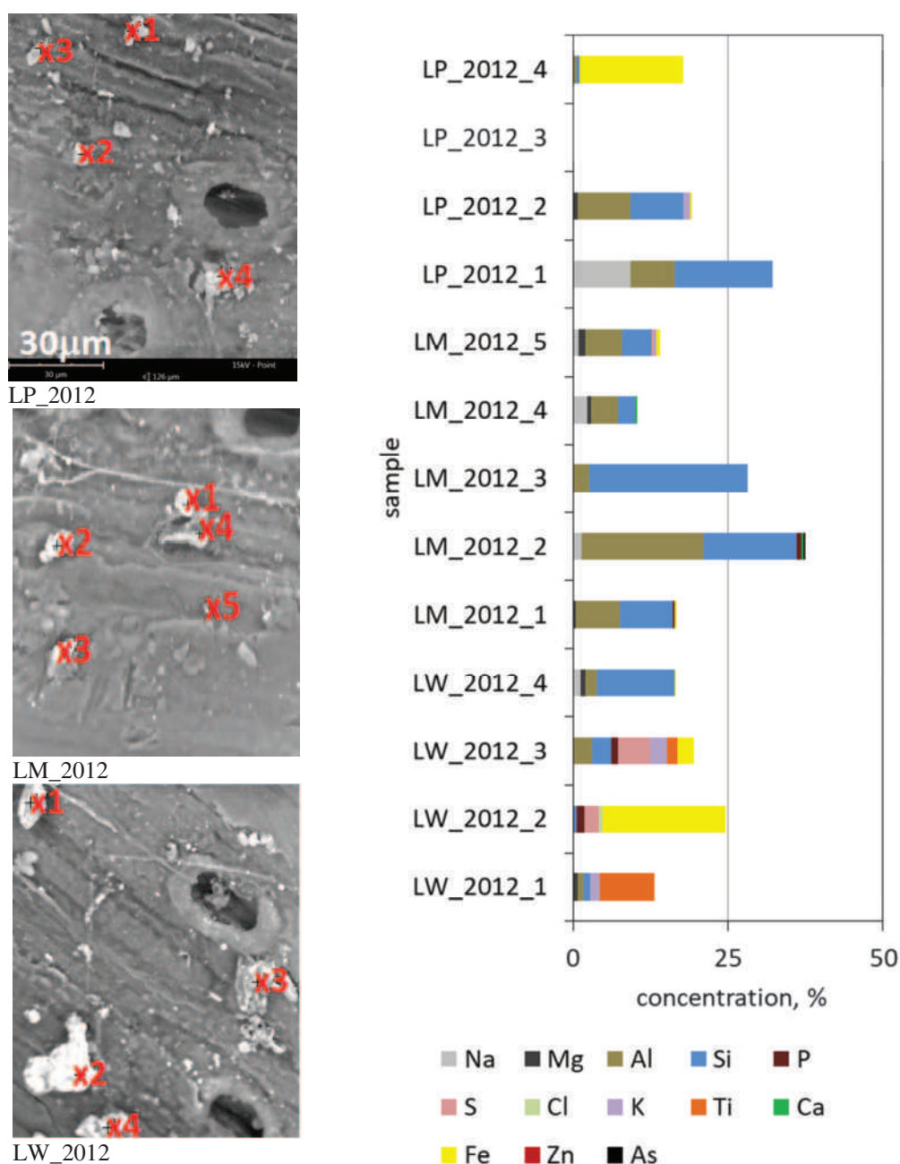
Figure 2: Micrographs of the surface of the needles and the elements and chemical compounds deposited on the needles in 3 cities: Wiry (LW), Mikołów (LM) and Podlesie (LP) in the area located nearby industrial factory Łaziska Power Station. The samples were created in 2012 (collected in January 2013). "x" mark the points of the surface in which the chemical composition was determined by SEM.
